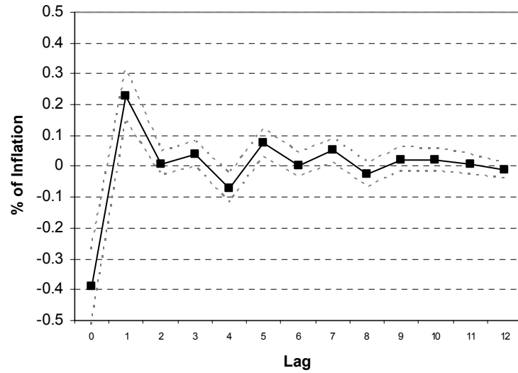
Panel A: Response of Inflation to a 1% Supply Shock
