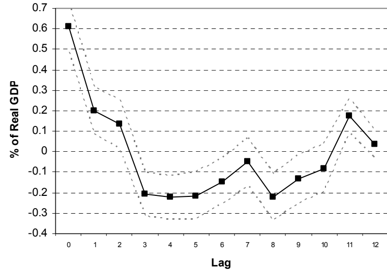
Panel B: Response of Output to a 1% Demand Shock
