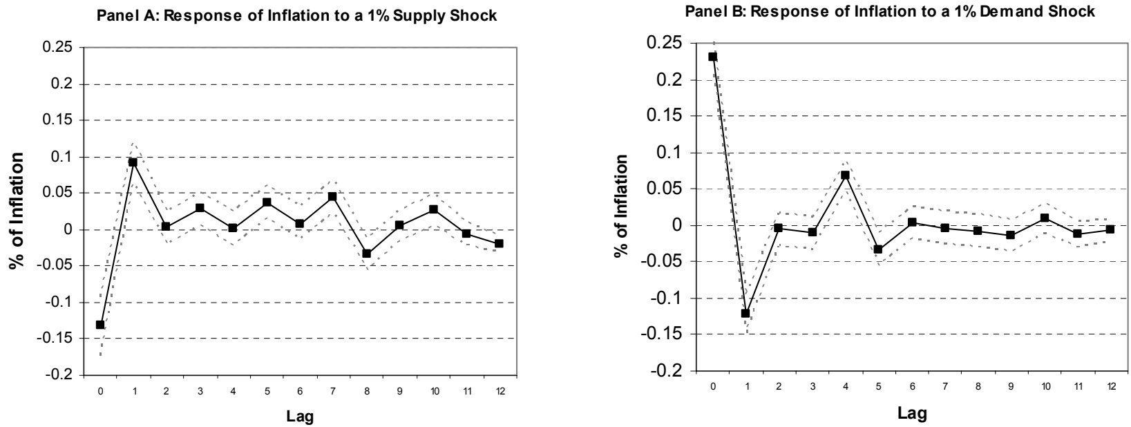
Figure 2: Inflation Responses with the B-Q Restrictions
