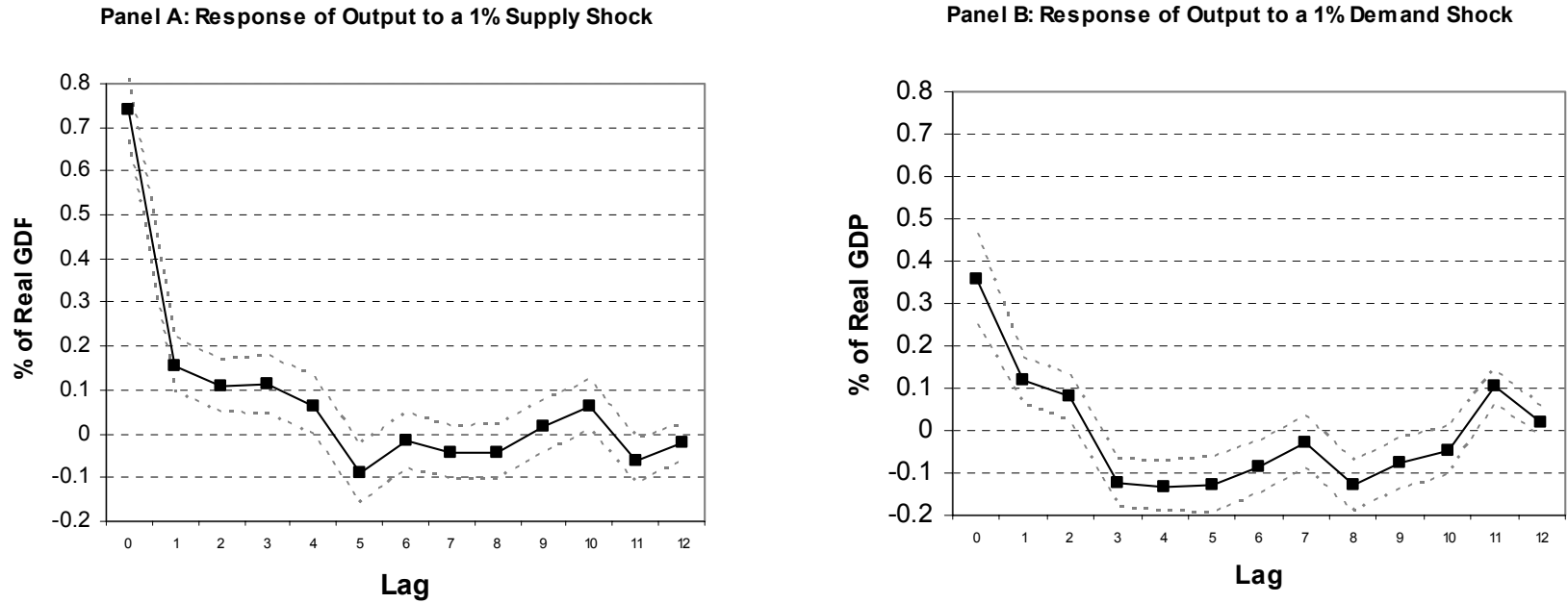
Figure 1: Output Responses with the B-Q Restrictions
