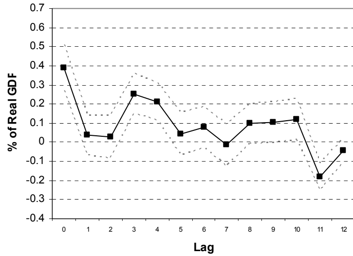
Panel A: Response of Output to a 1% Supply Shock
