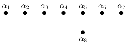
Figure 1. Coxeter Diagram for E_8 .
